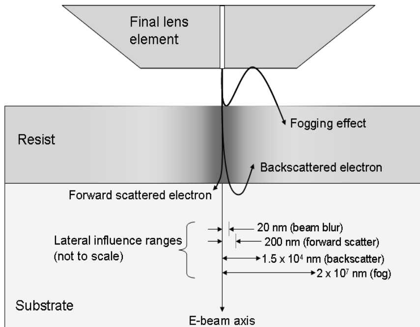
Figure 1: Electron beam – material interactions
