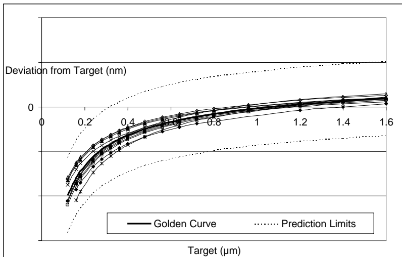
Figure 5: Comparing fitted curves for QA cell data from eleven masks to the Golden Curve.
