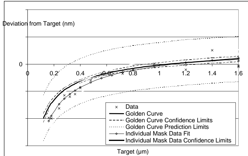
Figure 7: Comparing the confidence limits of the fit of an individual mask data set to that of the Golden Curve, created with significantly more data.
