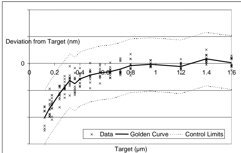
Figure 2: Golden Curve generated with point-by-point averaging
