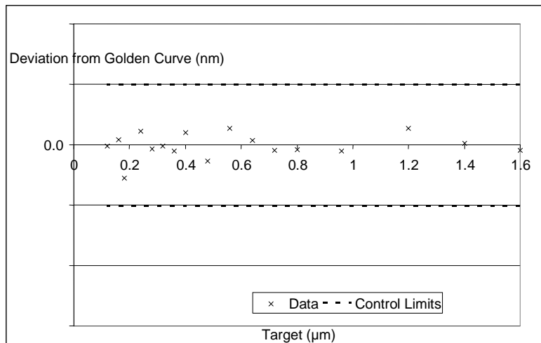
Figure 3: Comparing QA cell data from an individual mask to the Golden Curve. The point-by-point deviation from the Golden Curve is compared to control limits.
