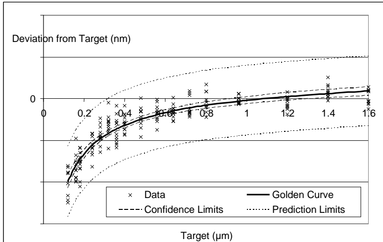
Figure 4: Golden Curve generated by fitting a function to representative data.
